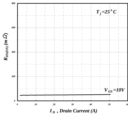
Fig 13. Typ. Drain-Source on State Resistance
