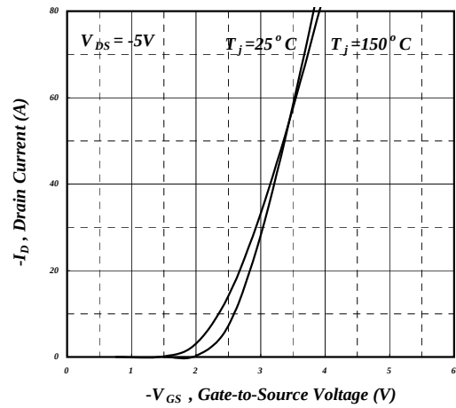
Fig 14. Transfer Characteristics
