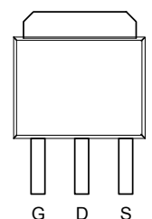
TO-251VS(JV)
