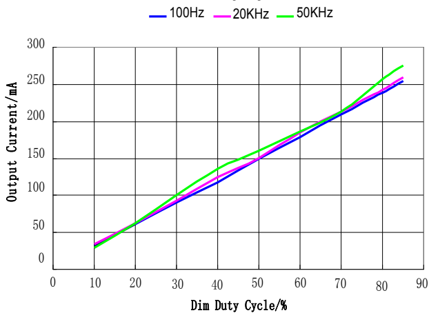
Iout vs Duty Cycle
