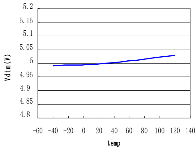
Vdim vs temperature
