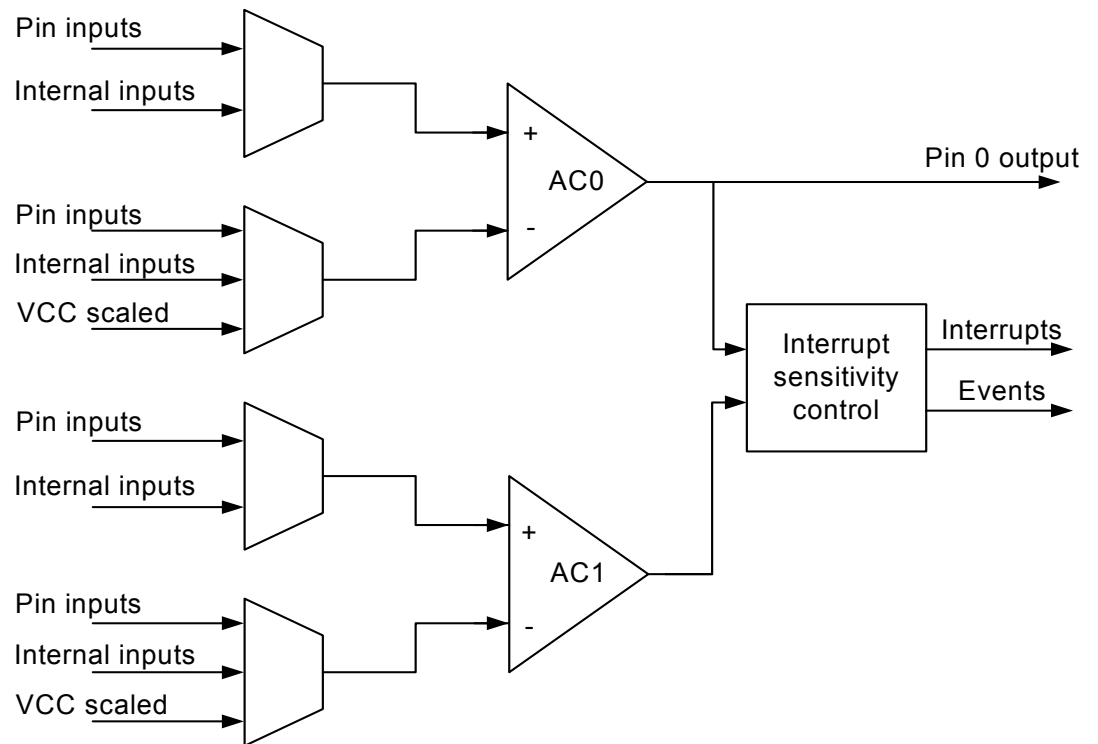
Figure 27-1. Analog Comparator overview.
