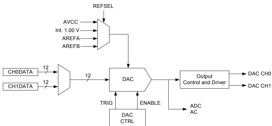
Figure 26-1. DAC overview
