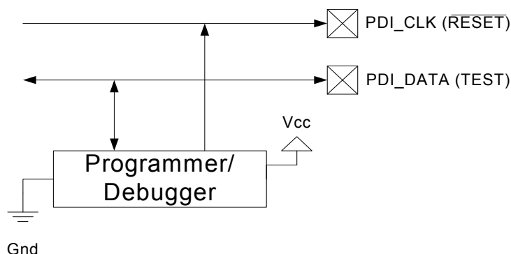
Figure 29-2. PDI connection
