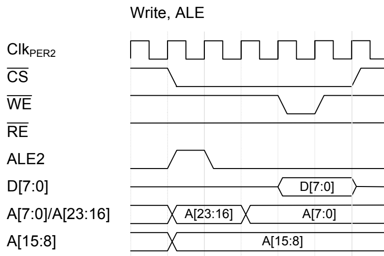
Figure 33-12. Write, ALE
