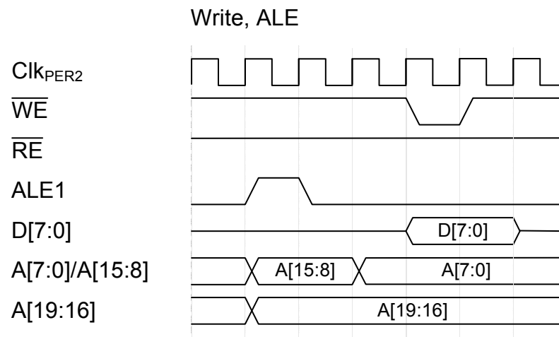
Figure 33-26. Write, ALE
