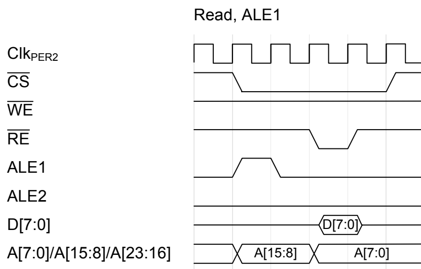
Figure 33-9. Read, ALE1
