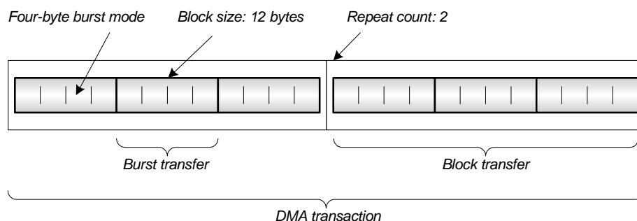
Figure 5-1. DMA transaction.
