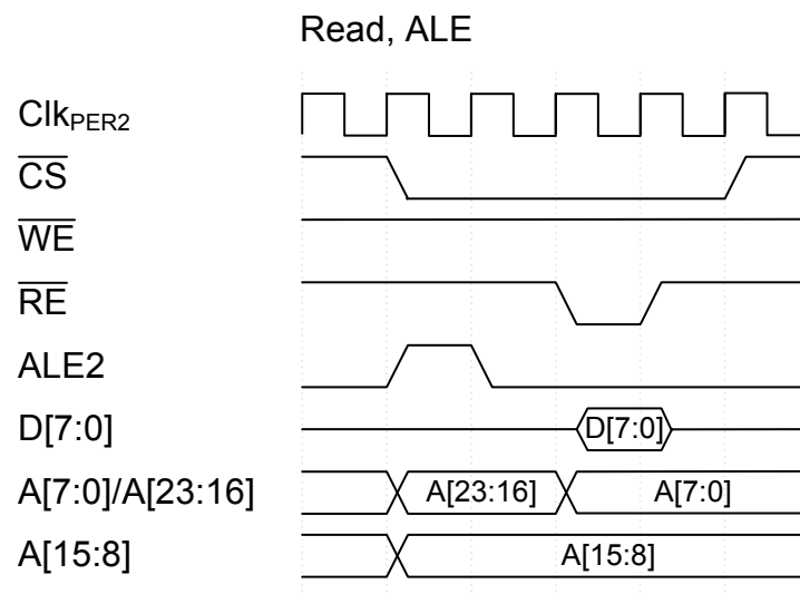
Figure 33-14. Read, ALE
