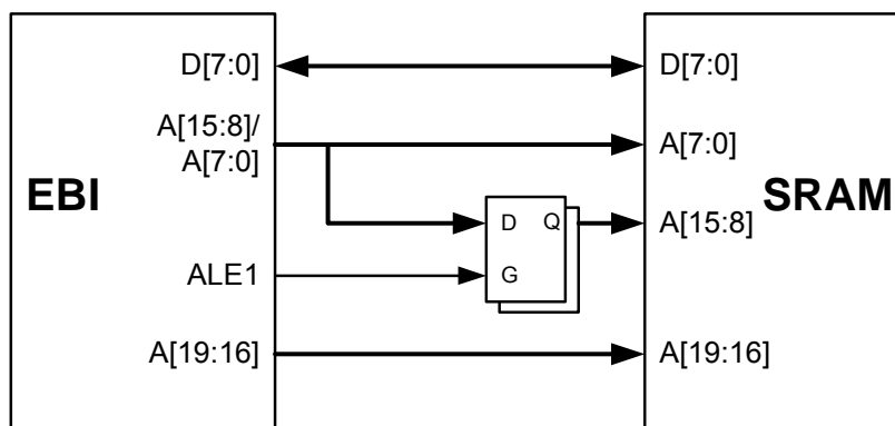
Figure 24-3. Multiplexed SRAM connection using ALE1
