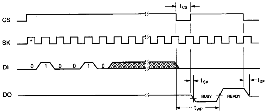
FIGURE 8. ERASE ALL (ERAL) CYCLE TIMING
