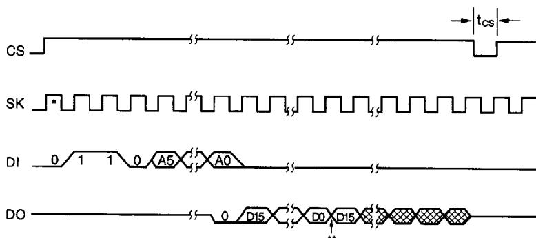
FIGURE 2. READ CYCLE TIMING
