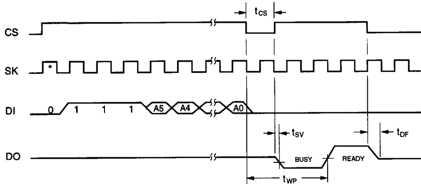
FIGURE 7. ERASE (REGISTER) CYCLE TIMING
