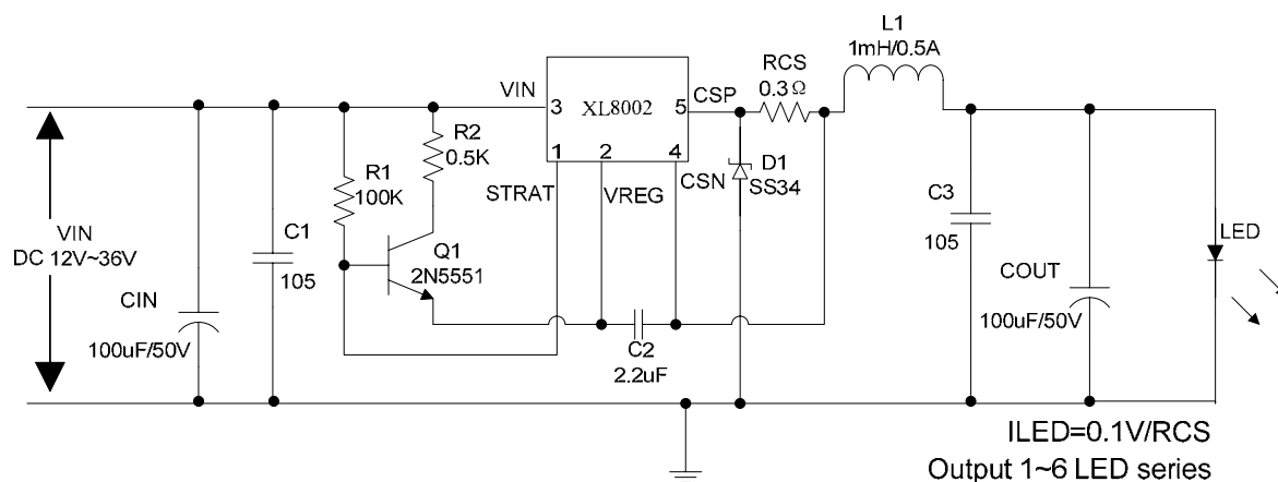
Figure11. XL8002 System Application at VIN=12V~36V Schematic
