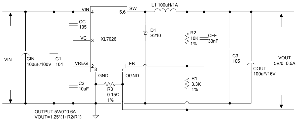
Figure9. XL7026 System Application (VOUT=5V, IOUT=0~0.6A)
