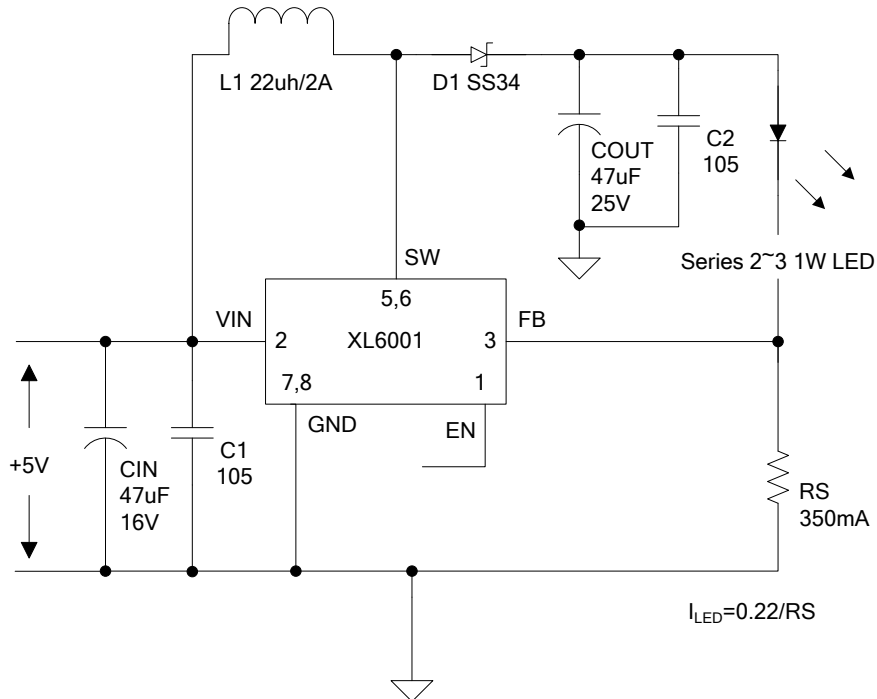
Figure5. XL6001 System Parameters Test Circuit (2~3 x 1W LED)
