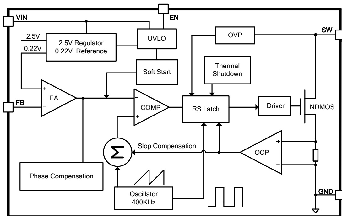
Figure3. Function Block Diagram of XL6001
