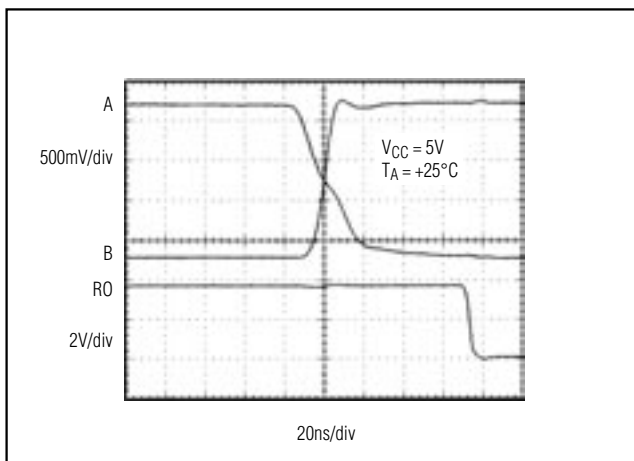
485 Receiver t_{PHL}
