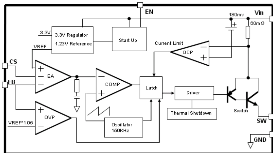
Figure3. Function Block Diagram of XL4011
