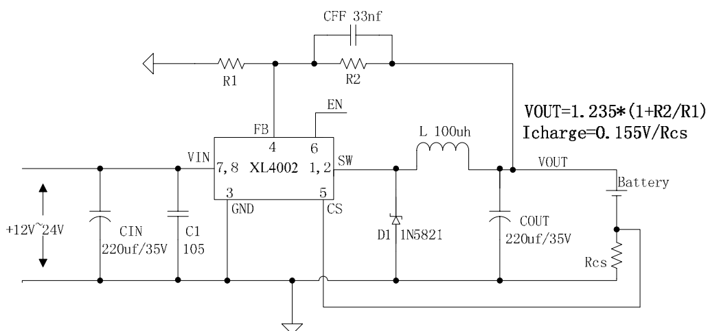
Figure4. XL4002 Typical Application Circuit (Li Battery Charger)
