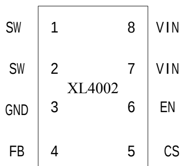
Figure2. Pin Configuration of XL4002 (Top View)
