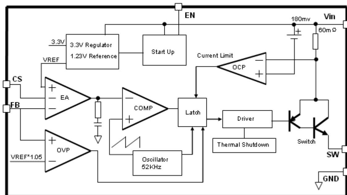
Figure3. Function Block Diagram of XL4002
