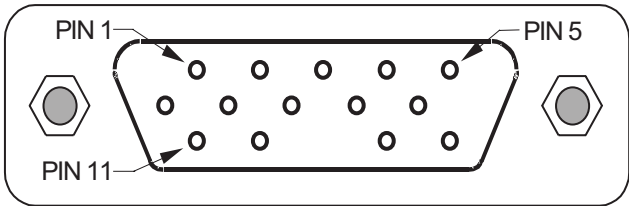
FIGURE 1 VGA CONNECTOR LAYOUT
