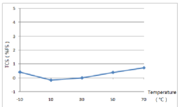
TCS-Constant Current
