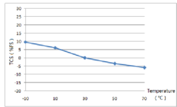
TCS-Constant Voltage
