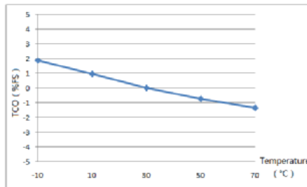
TCO-Constant Voltage
