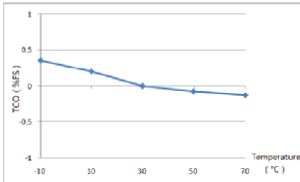
TCO-Constant Current
