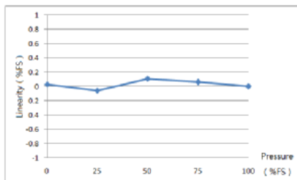
Linearity
