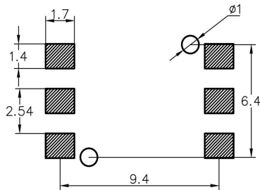
XGZP160-SOP Type
