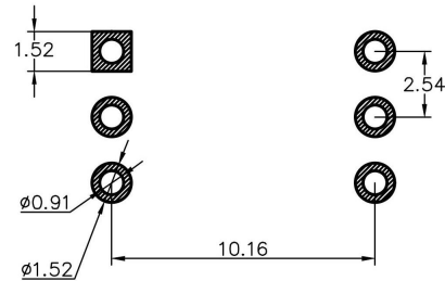
XGZP160-DIP Type
