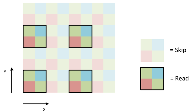
Figure 7. Color Subsampling (Read-2-Skip-2)
