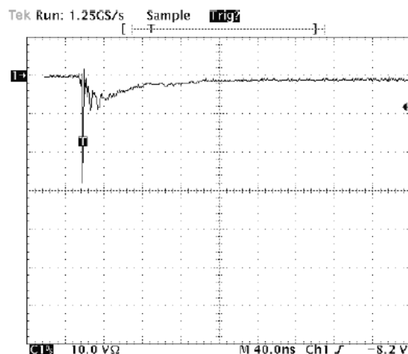
Fig 5. Negative 8kV contact per IEC 61000-4-2
