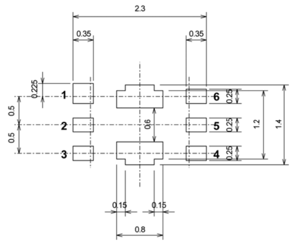
USP-6B Reference Metal Mask Design
