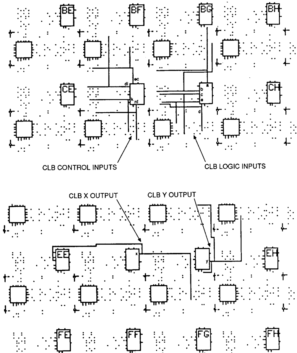
Figure 9: Design Editor Locations of interconnect access, CLB control inputs, logic inputs and outputs. The dot pattern represents the available programmable interconnection points (PIPs).
