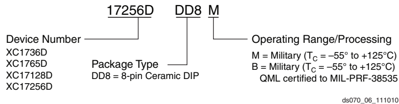
Figure 6: Marking Information
