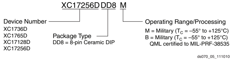
Figure 5: Ordering Information
