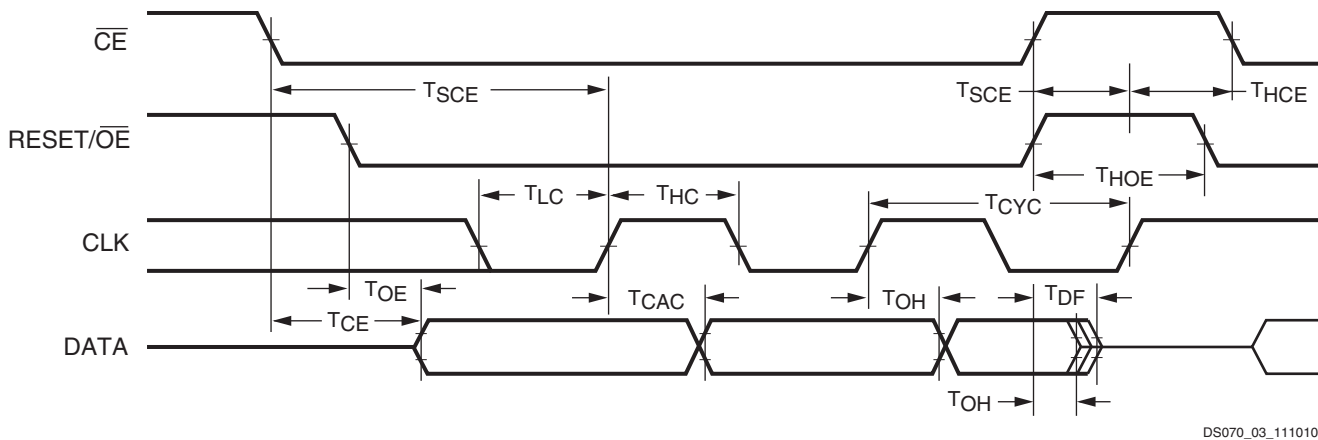
Figure 3: AC Characteristics Over Operating Condition
