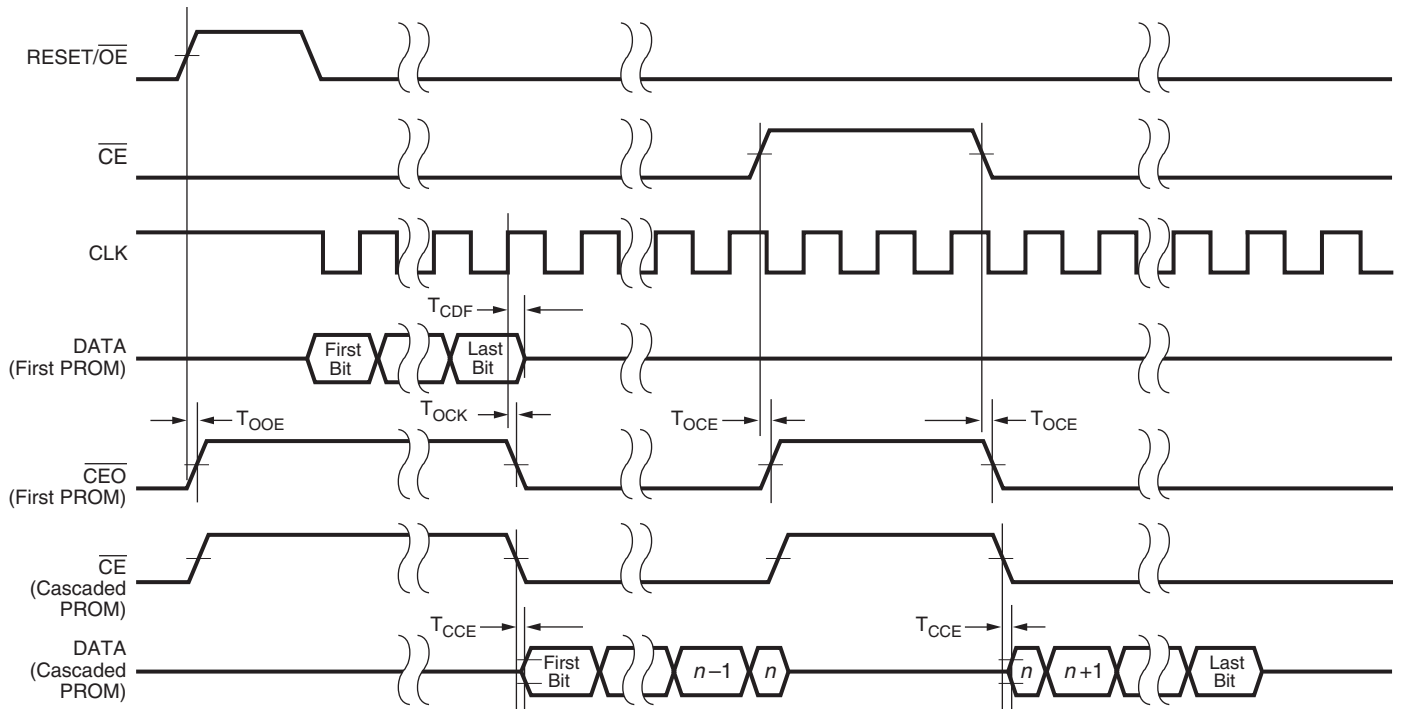
Figure 4: AC Characteristics Over Operating Condition When Cascading
