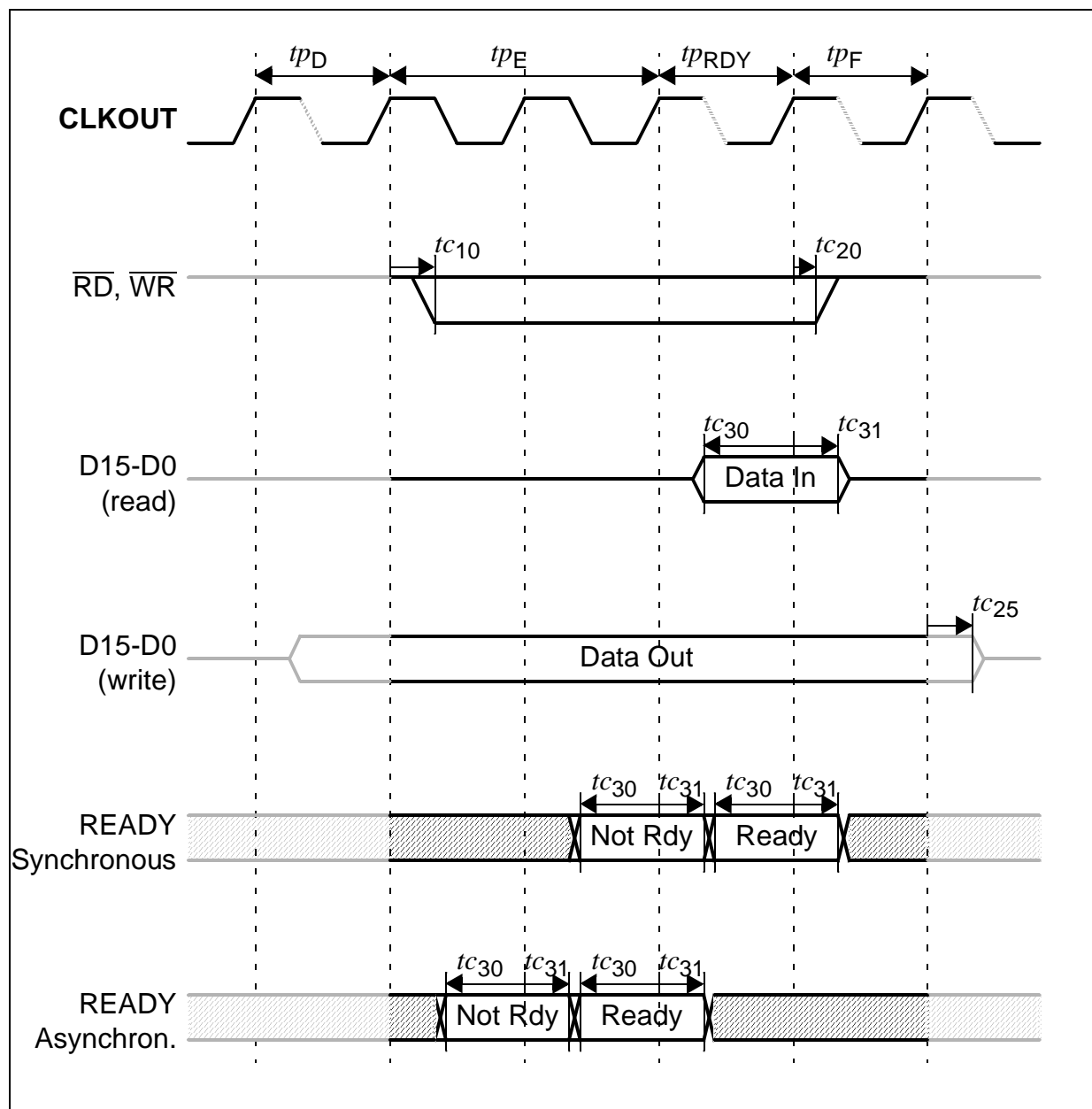
Figure 23 READY Timing
