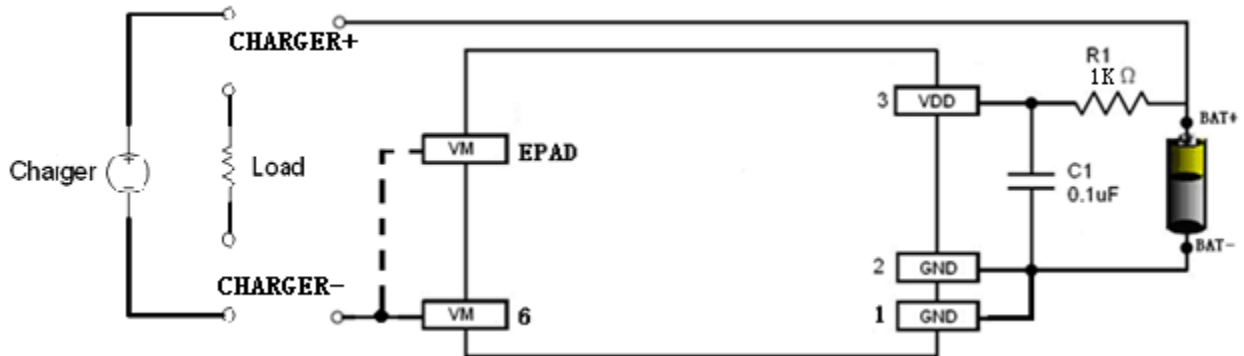
Fig 6 XB9501G in a Typical Battery Protection Circuit
