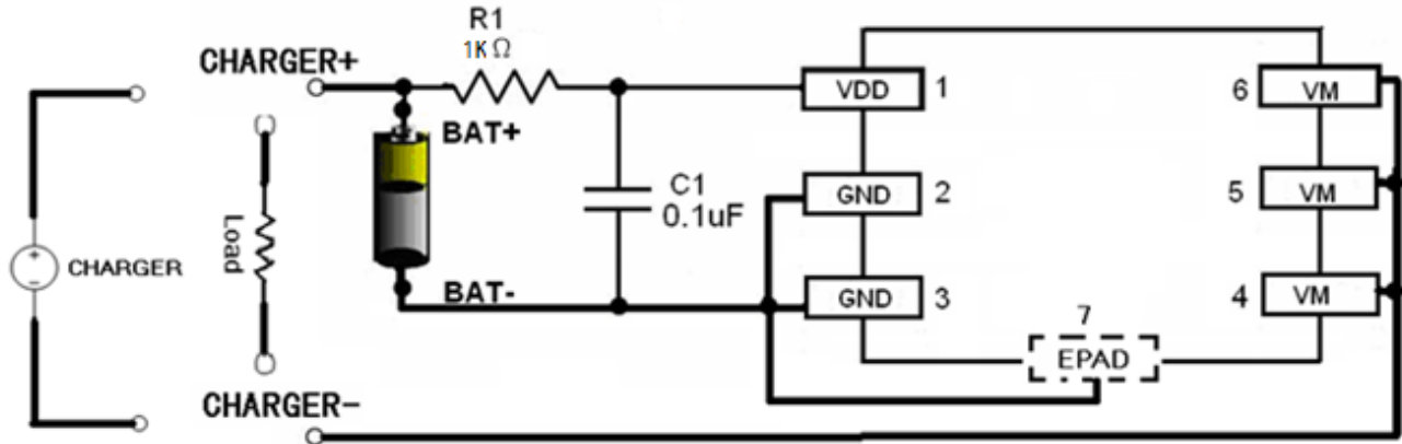
Fig 6 XB6166J4S in a Typical Battery Protection Circuit
