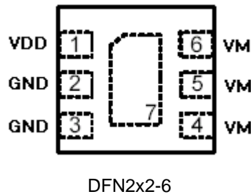
Figure 2. PIN Configuration
