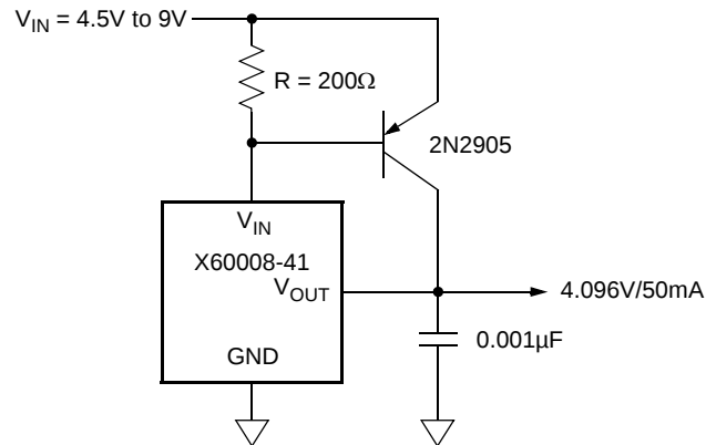
Precision 4.096V, 50mA Reference.
