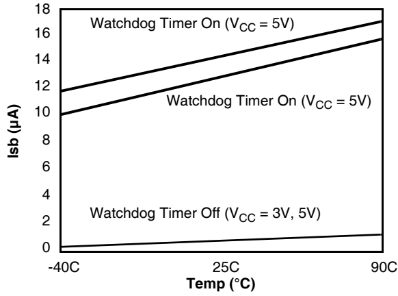
V_{CC} Supply Current vs. Temperature ( I_{SB} )
