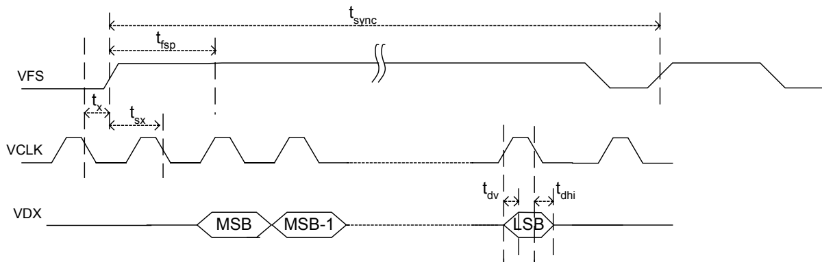
Figure 23. CODEC Timing -- Long Frame Sync.
