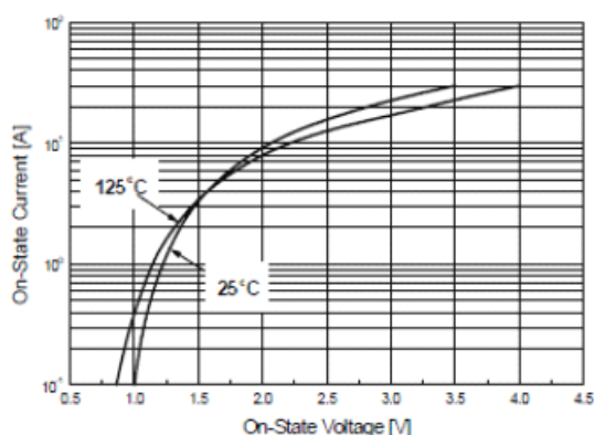
Fig.2 On-State Voltage
