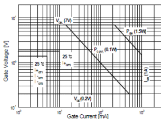
Fig1. Gate Characteristics
