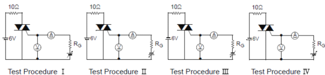
Fig.9 Gate Trigger Characteristics Test Circuit
