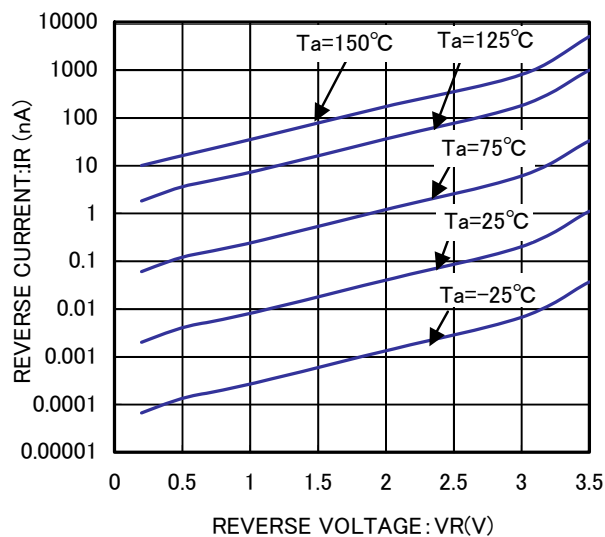
Fig-2 V_R - I_R CHARACTERISTICS
