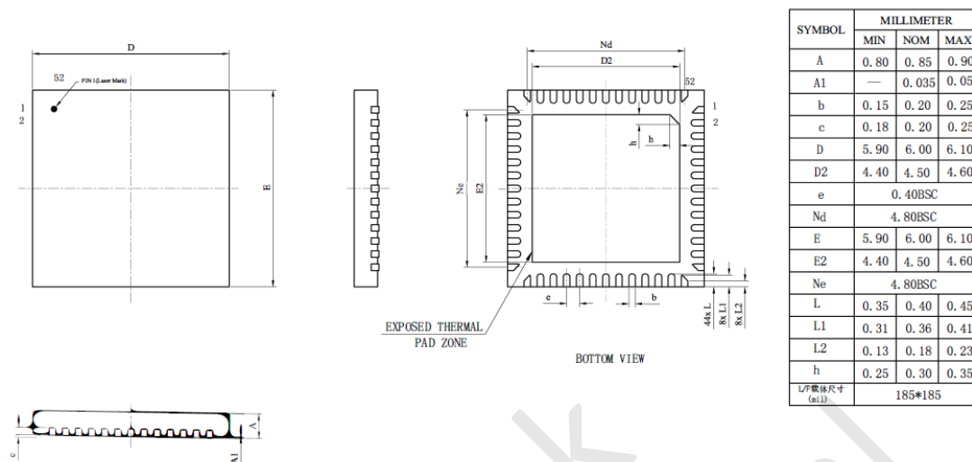
Figure 7-1 WS300 Package
