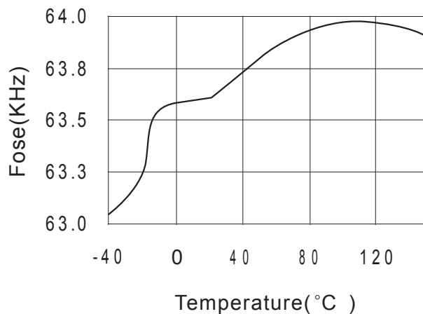
Fose(KHz) vs Temperature ( ^{\circ} C )
