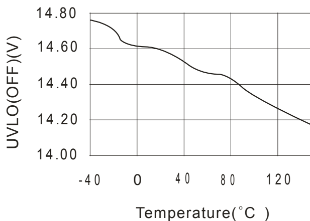
UVLO(OFF)(V) vs Temperature( ^{\circ} C )
