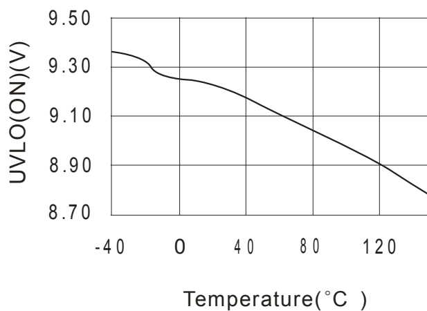
UVLO(ON)(V) vs Temperature( ^{\circ} C )
