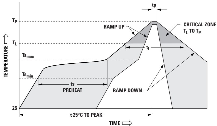
Figure 19. Typical SMT reflow profile for maximum temperature = 260 \pm 0/-5^\circ\text{C}
