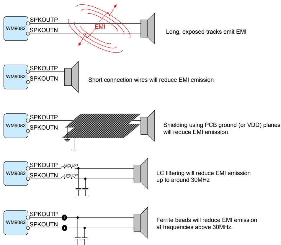
Figure 8 EMI Reduction Techniques
