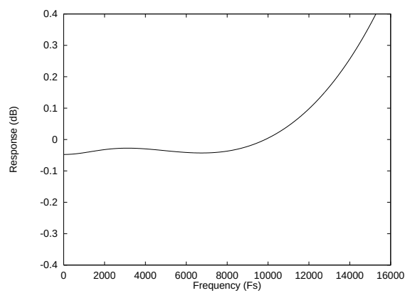
Figure 37 De-emphasis Error (32kHz)
