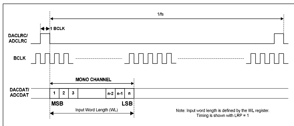
Figure 16 DSP Mode Audio Interface (mode A, LRP=0)
