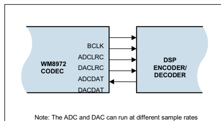
Figure 11 Master Mode
