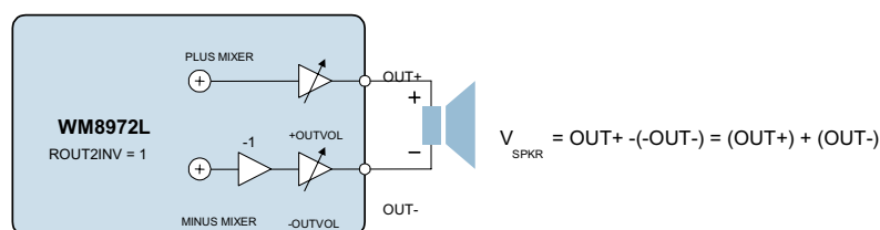
Figure 9 Speaker Output Connection
