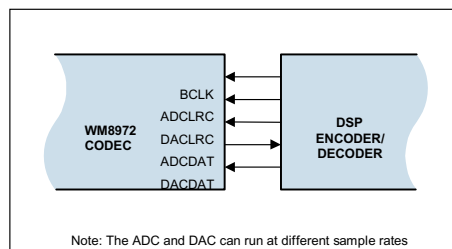
Figure 12 Slave Mode
