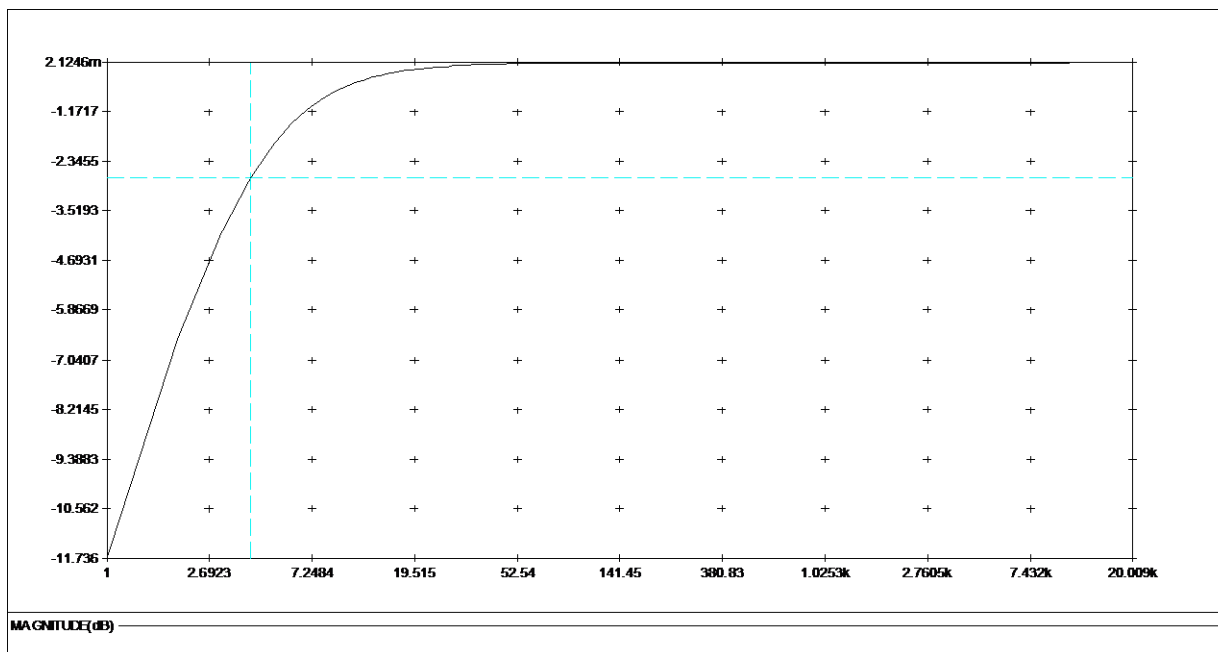
Figure 85 ADC Digital High Pass Filter Frequency Response (48kHz, Hi-Fi Mode, ADC_HPF_CUT[1:0]=00)
