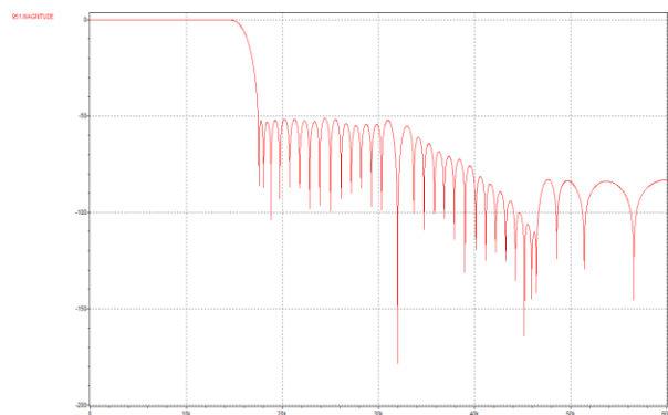
Figure 79 DAC Playback Filter Response for 32k Sample Rate
