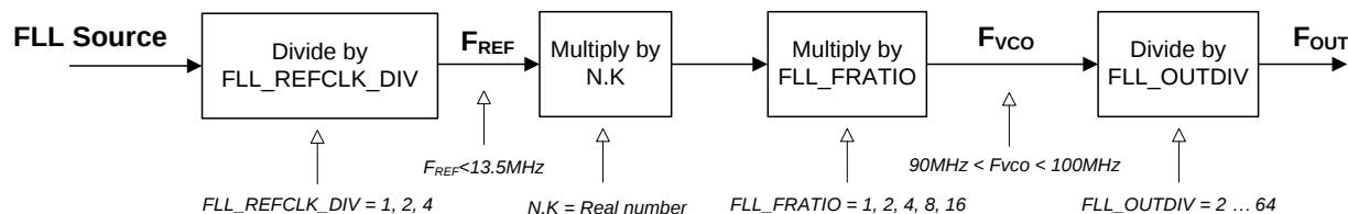
Figure 59 FLL Configuration
