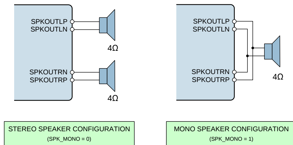
Figure 33 Mono and Stereo Speaker Output Configuration
