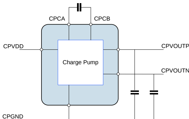
Figure 36 Charge Pump External Connections
