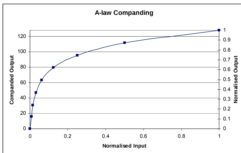
Figure 32 A-Law Companding
