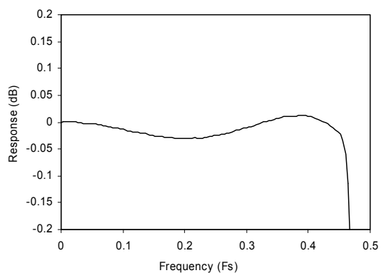
Figure 39 DAC Digital Filter Ripple
