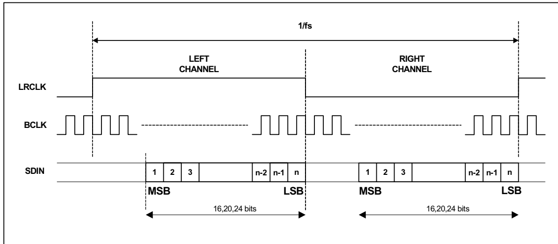
Figure 16 MSB First Right-justified Data Input
