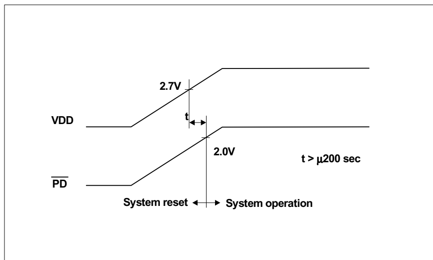
Figure 3 \overline{\text{PD}} Pin Levels at Power On
