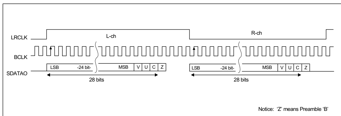
Figure 13 Data Output Timing – NRZ Data LSB First Left-justified Output
