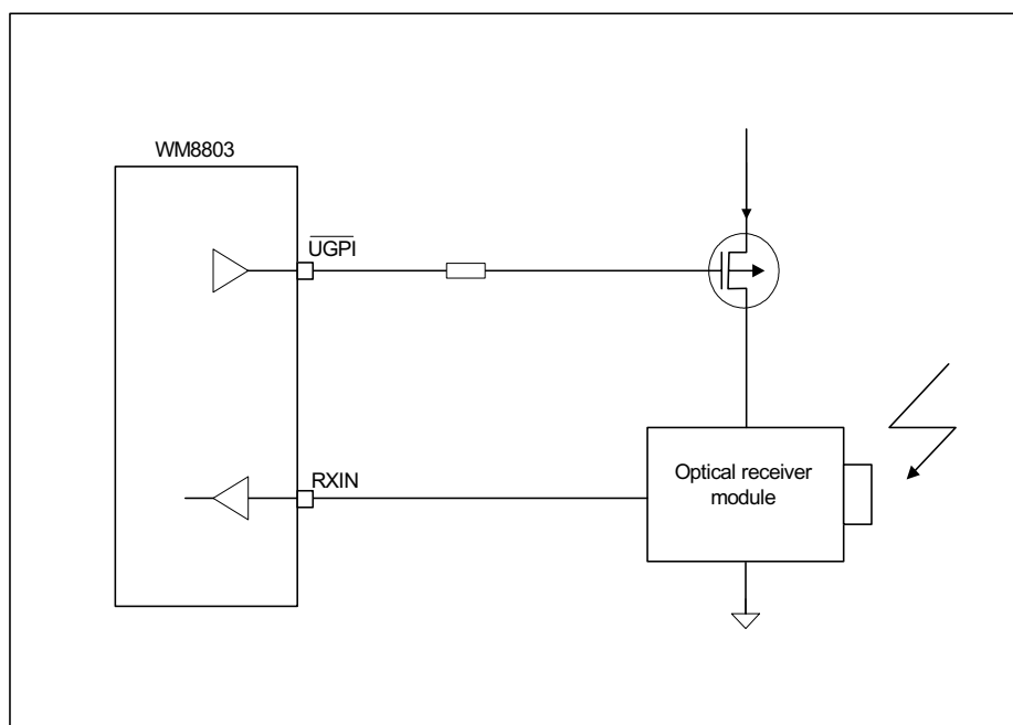
Figure 20 \overline{\text{UGPI}} Output Example (Optical Receiver Module Power Supply Control)
