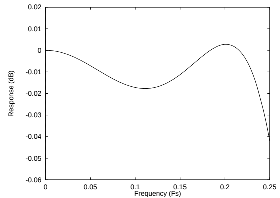
Figure 37 DAC Digital Filter Ripple – Type 2
