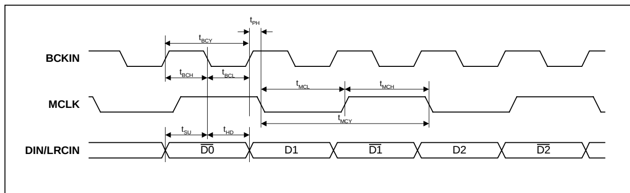
Figure 4 Biphas DSD Timing Requirements
