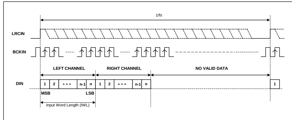
Figure 11 DSP Late Mode Timing Diagram
