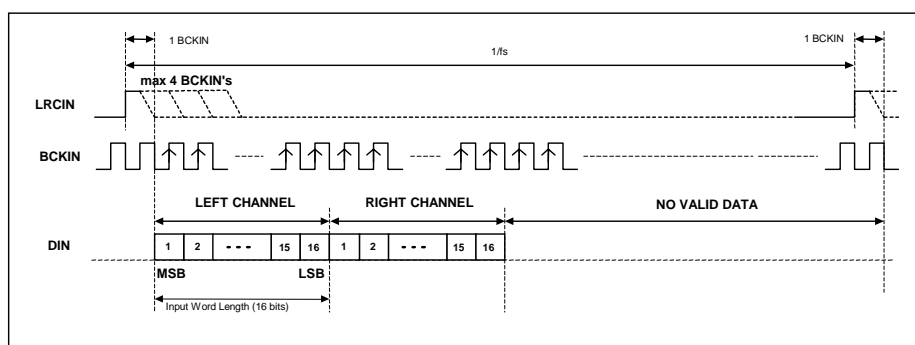
Figure 8 DSP Mode A Timing
