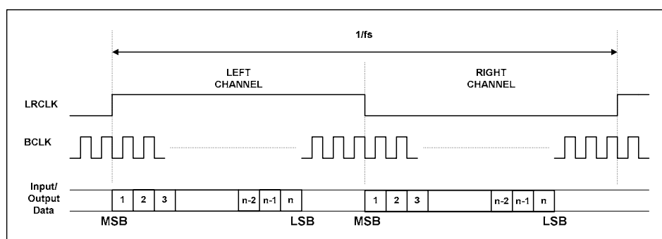
Figure 14 Left Justified Mode Timing Diagram
