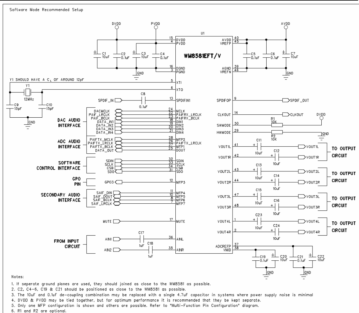
Figure 49 Recommended-External Components - Software
