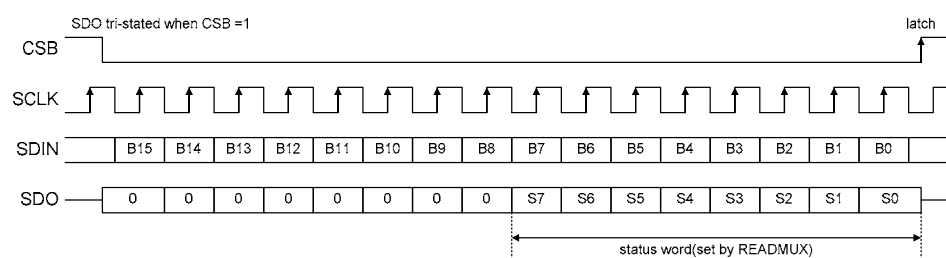
Figure 7 3-Wire SPI Compatible Interface Continuous Readback
