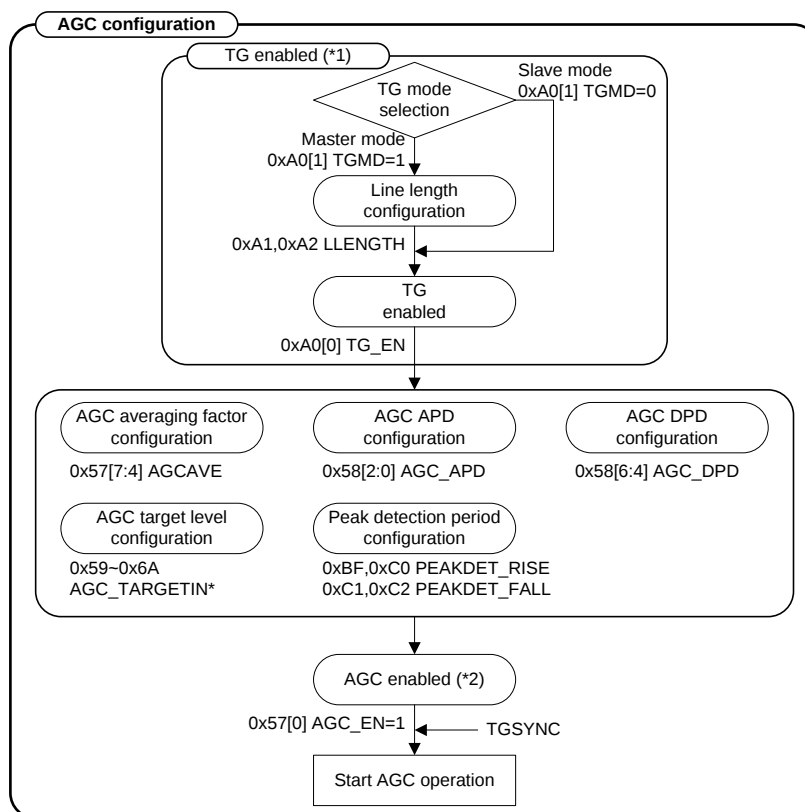
Figure 47 AGC Configuration
