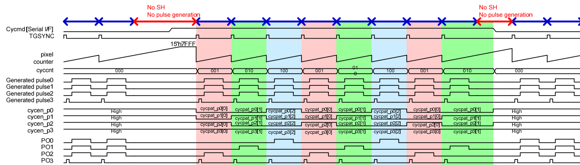
Figure 21 TG Cycle Mode
