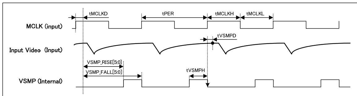
Figure 6 Input Video Timing (SH mode)
