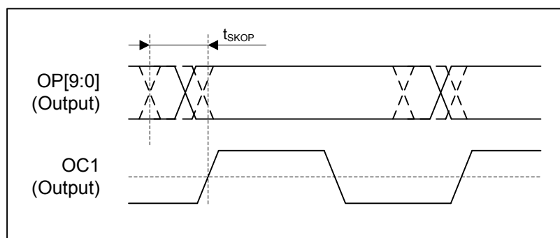
Figure 8 CMOS Output Data Timing
