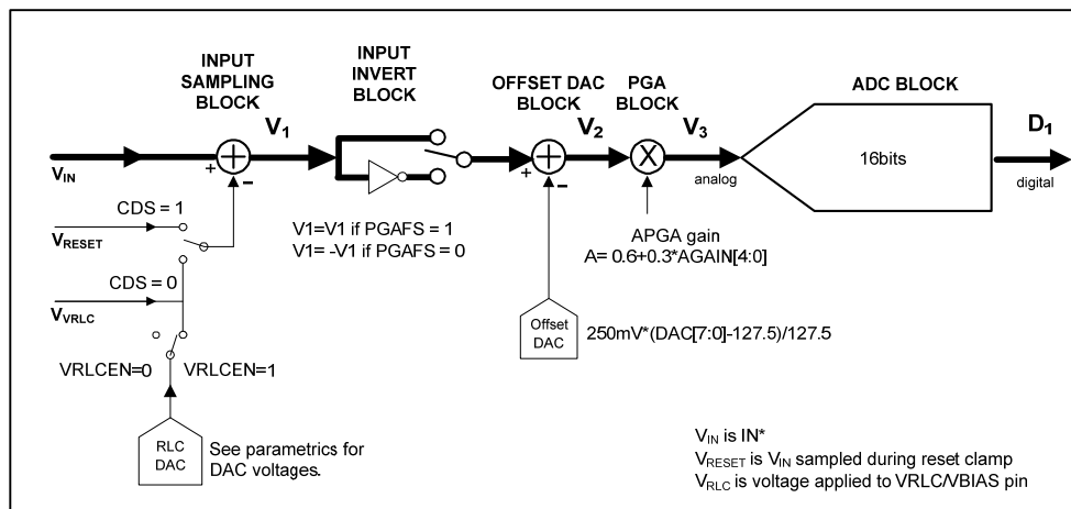
Figure 15 Overall Signal Flow
