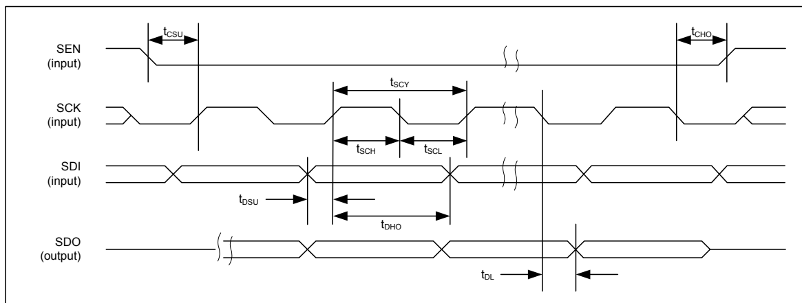
Figure 3 Serial Interface Timing
