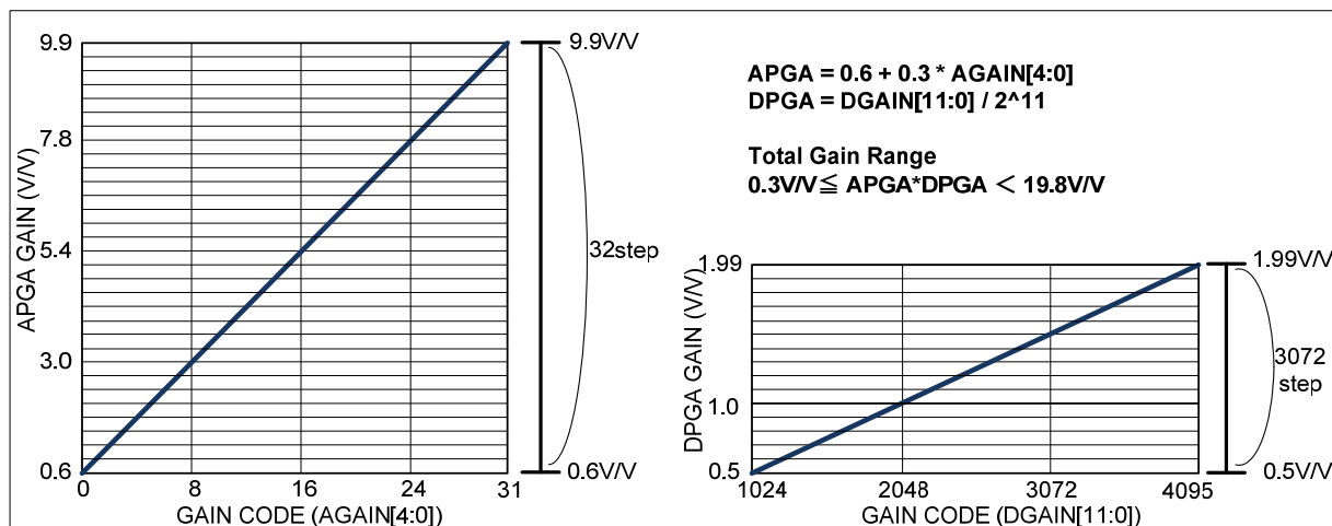
Figure 13 PGA Gain Characteristic
