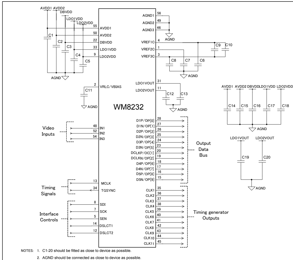
Figure 28 External Components Diagram
