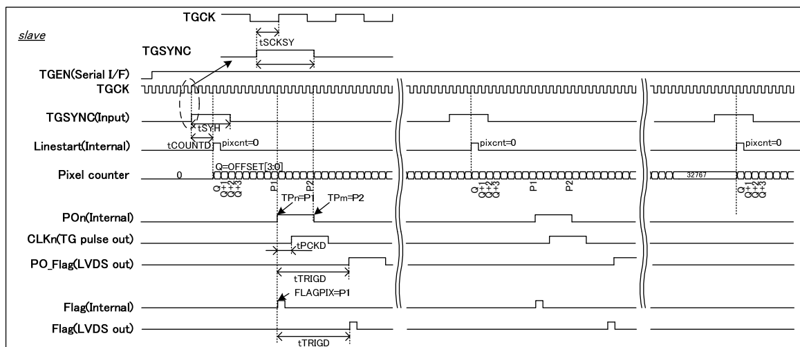
Figure 18 Slave Mode Pixel Counter and Line Start Timing
