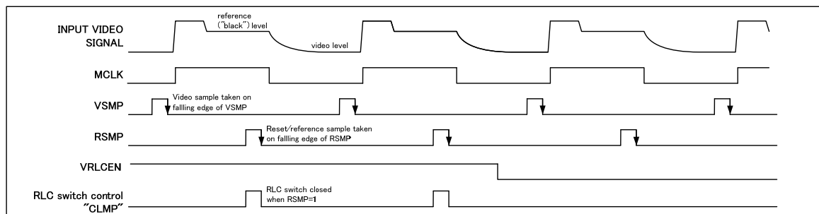
Figure 11 Reset Level Clamp Operation, CDS Operation Shown, non-CDS also Possible
