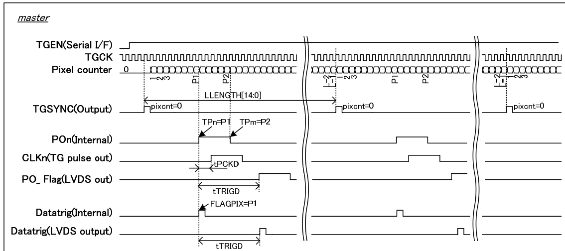
Figure 17 Master Mode Pixel Counter and Line Start Timing
