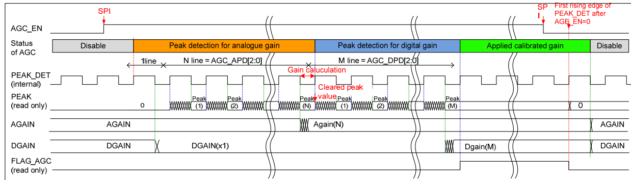
Figure 27 Automatic Gain Control
