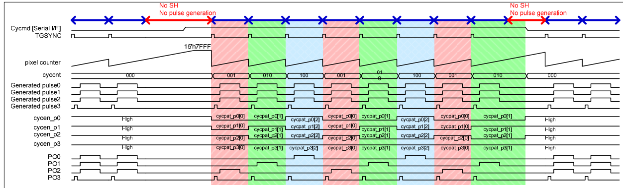
Figure 21 TG Cycle Mode
