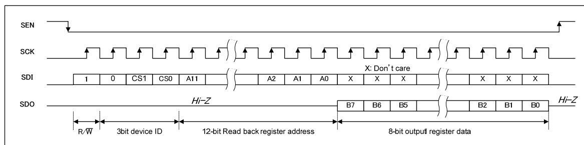
Figure 5 Serial Interface Register Read-back
