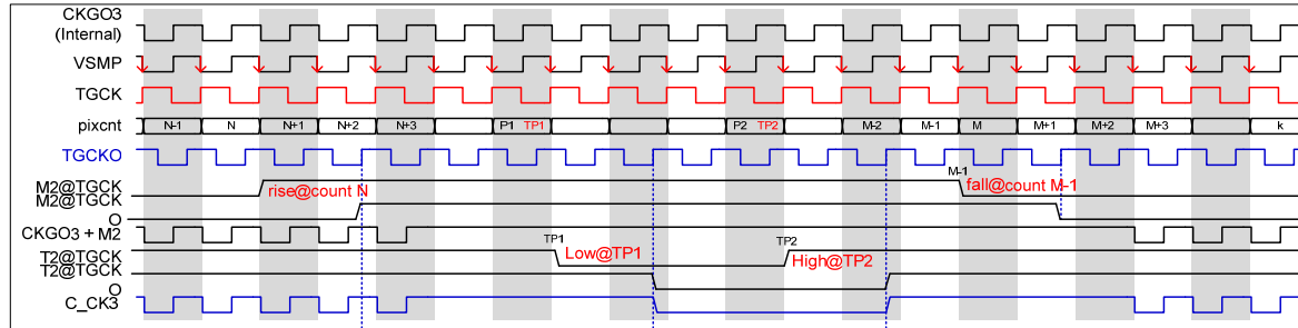
Figure 20 TG Mask Timing
