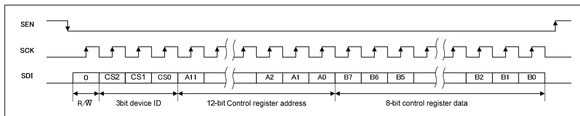
Figure 4 Serial Interface Register Write
