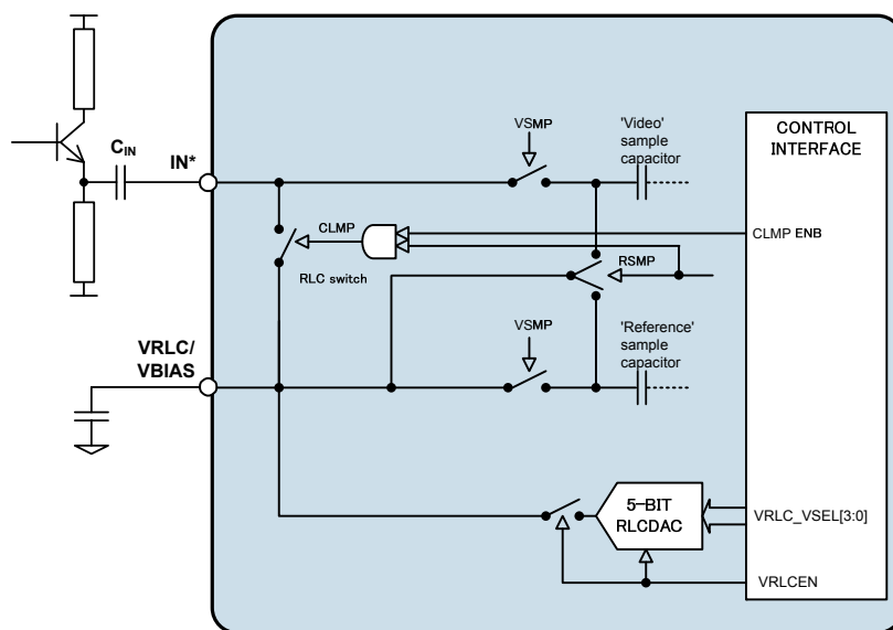
Figure 12 CDS/non-CDS Input Configuration
