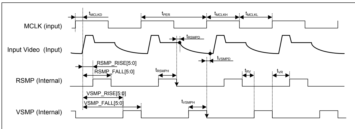
Figure 7 Input Video Timing (CDS mode)
