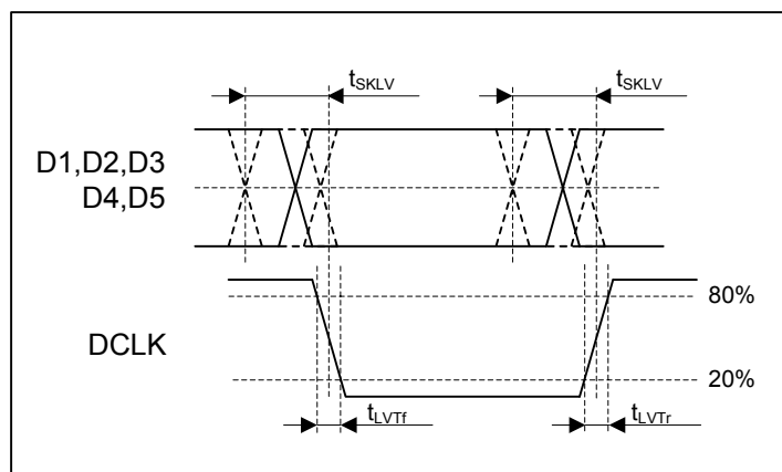
Figure 9 CMOS Output Data Timing
