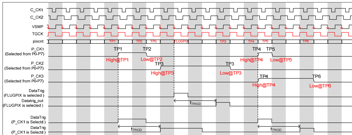
Figure 19 TG Pulse Toggle Setting and Data Trigger Timing
