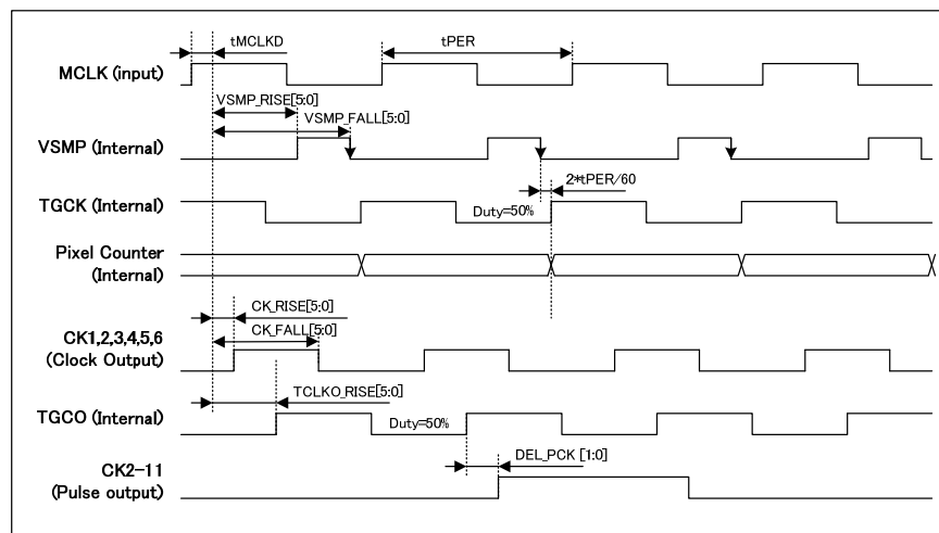
Figure 16 TG Output Timing
