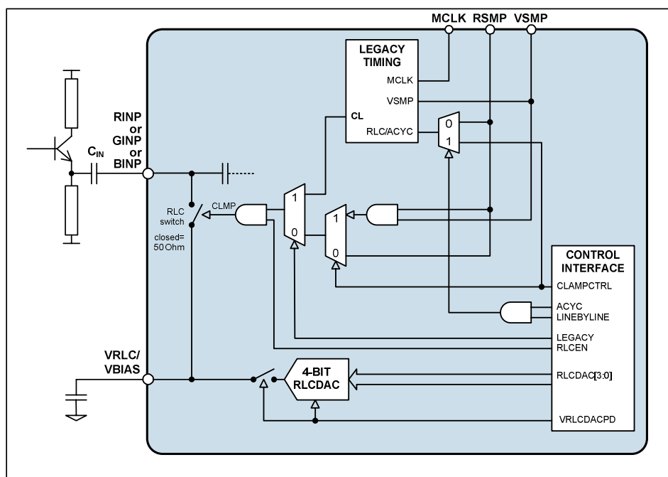
Figure 8 RLC Clamp Control Options
