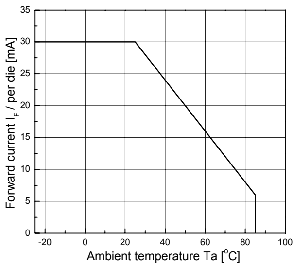
Forward Current Derating Curve (per die)
