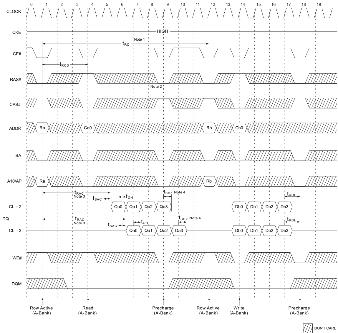
FIG. 5 READ &amp; WRITE CYCLE AT SAME BANK @BURST LENGTH=4
