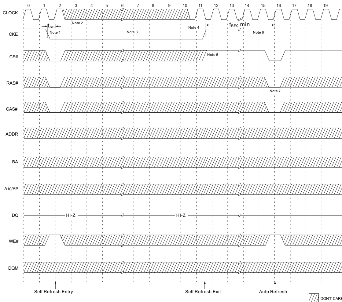
FIG. 16 SELF REFRESH ENTRY &amp; EXIT CYCLE
