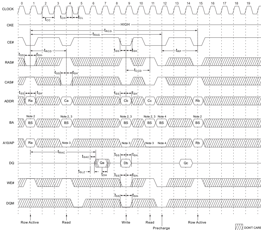
FIG. 3 SINGLE BIT READ-WRITE CYCLE (SAME PAGE) @CAS LATENCY=3, BURST LENGTH=1
