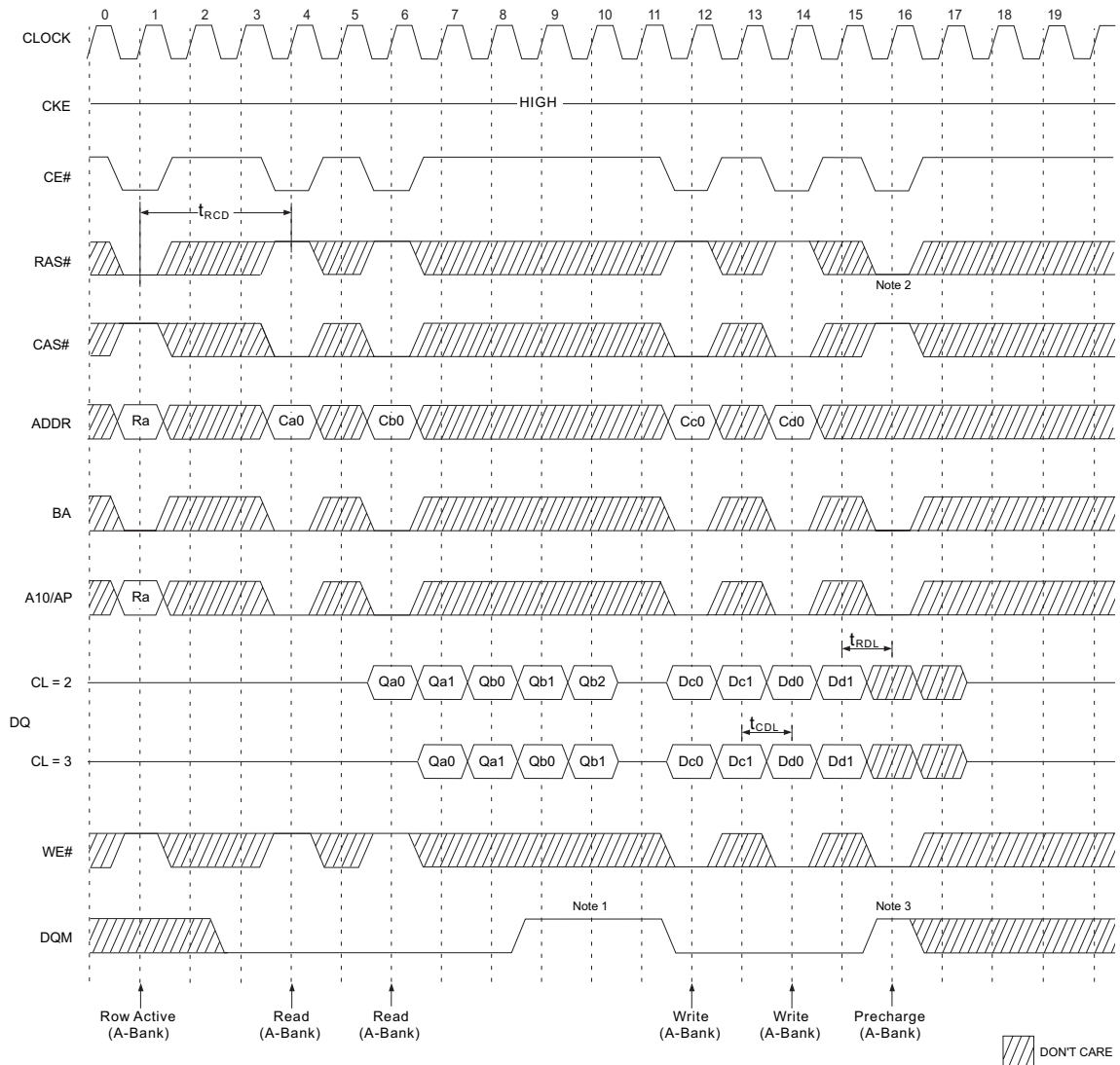
FIG. 6 PAGE READ &amp; WRITE CYCLE AT SAME BANK @BURST LENGTH=4
