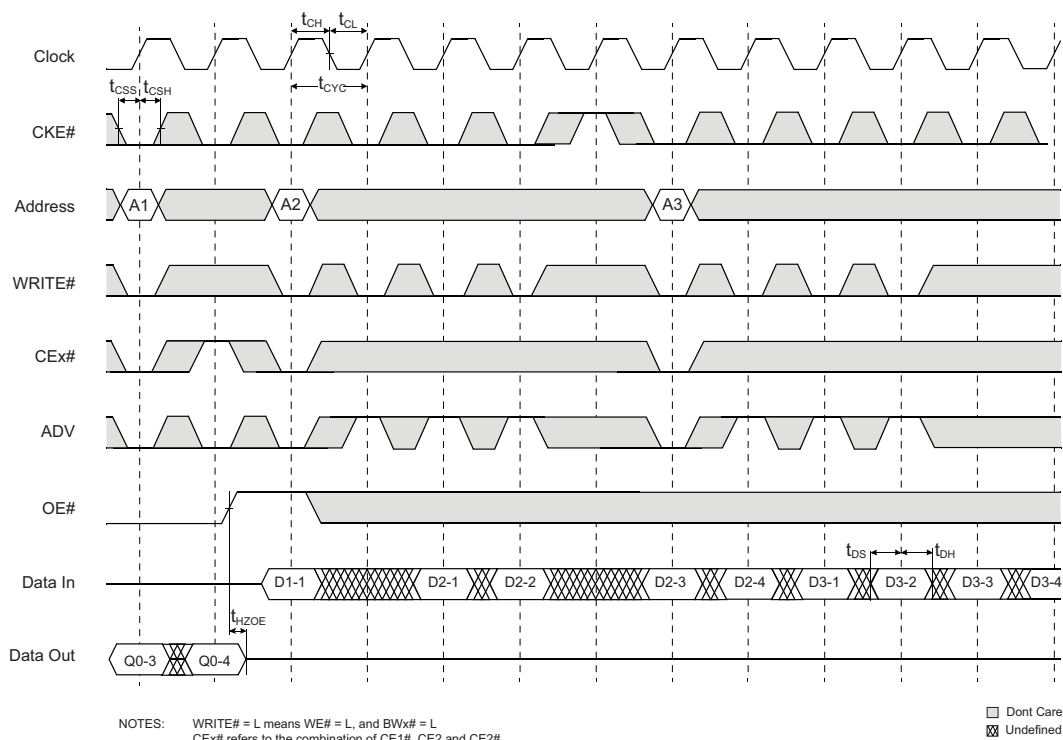
FIG. 4 TIMING WAVEFORM OF WRITE CYCLE
