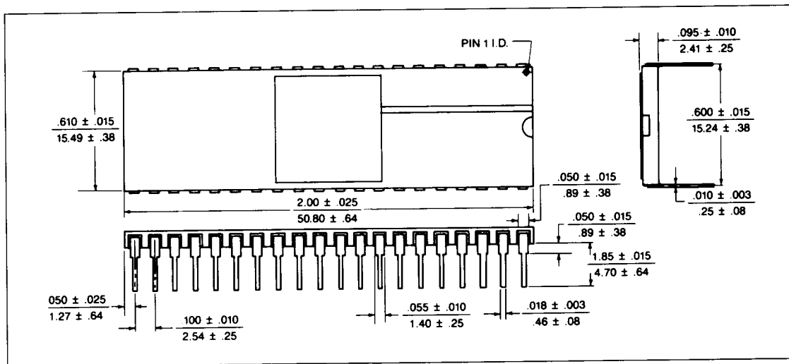
40 LEAD CERAMIC "AL"
