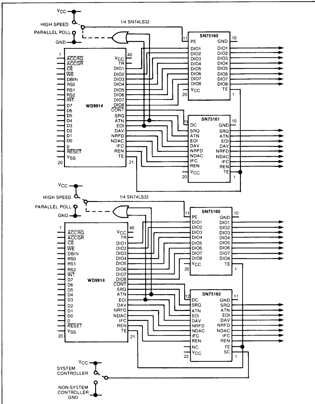
Figure 3. TRANSCEIVER CONNECTIONS
