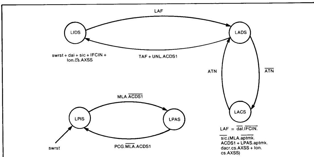
Figure 7. WD9914 LISTENER STATE DIAGRAM
