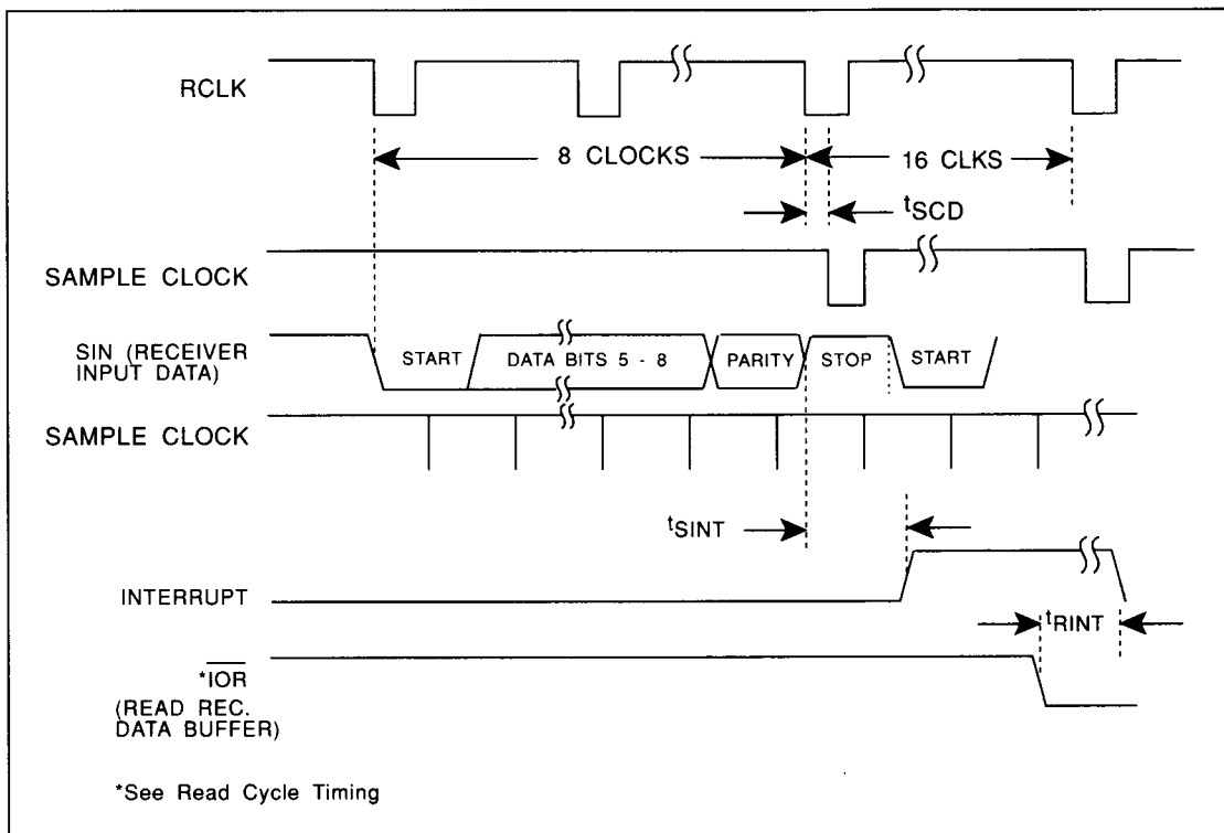
FIGURE 6-1. RECEIVER TIMING
