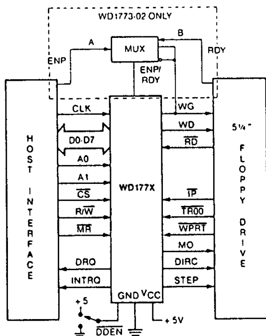
WD177X-02 SYSTEM BLOCK DIAGRAM
